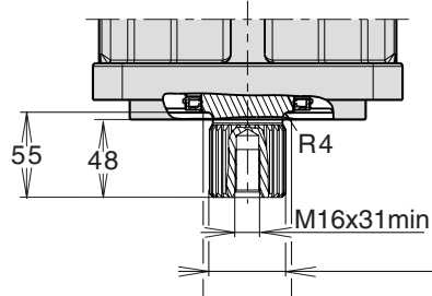
Type D spline shaft W50x24x9g DIN 5480 side fit
