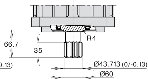
Type S spline shaft SAE J498b, class 1; 30° involute spline; 13T-8/16 DP; flat root, side fit
