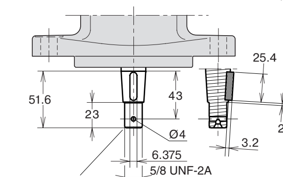
Tapered key shaft "V" SAE J744 22-3 (B)
