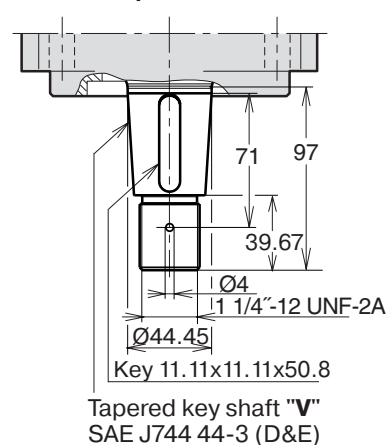
Shaft option V (F12-60)
