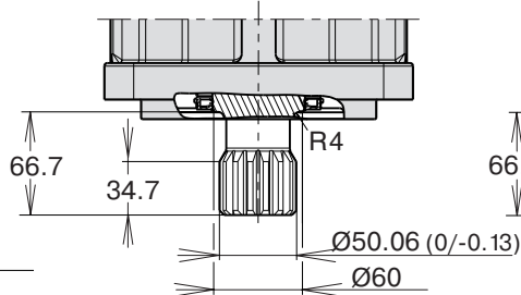
Type F spline shaft SAE J498b, class 1; 15T-8/16 DP; fillet root, side fit
