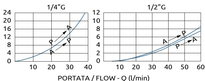
CURVE CARATTERISTICHE PERFORMANCE CURVES
